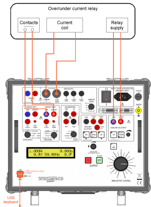
Figure 3.4 Connections for current drop-off test (with storage of result)
