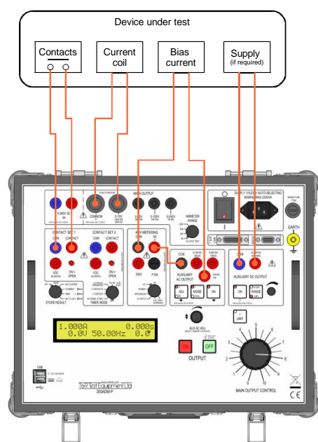
Figure 2.5 2 ac currents
