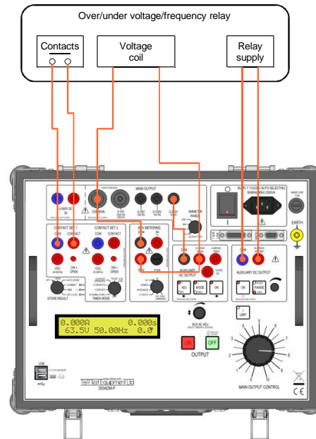
Figure 2.7 Voltage step
