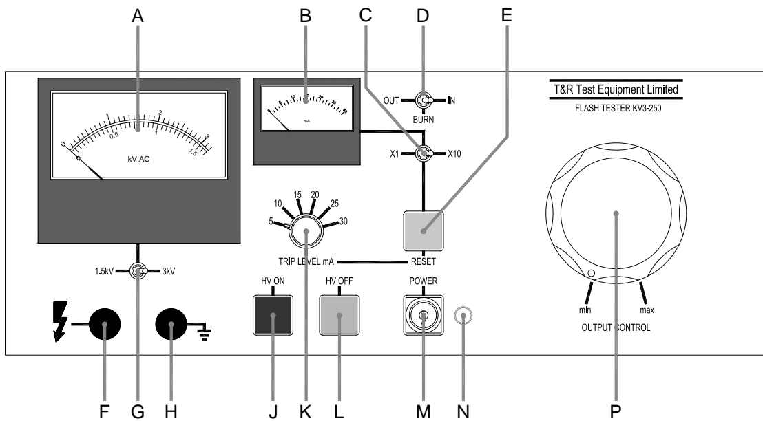
Figure 2.2 KV3-250 front panel
