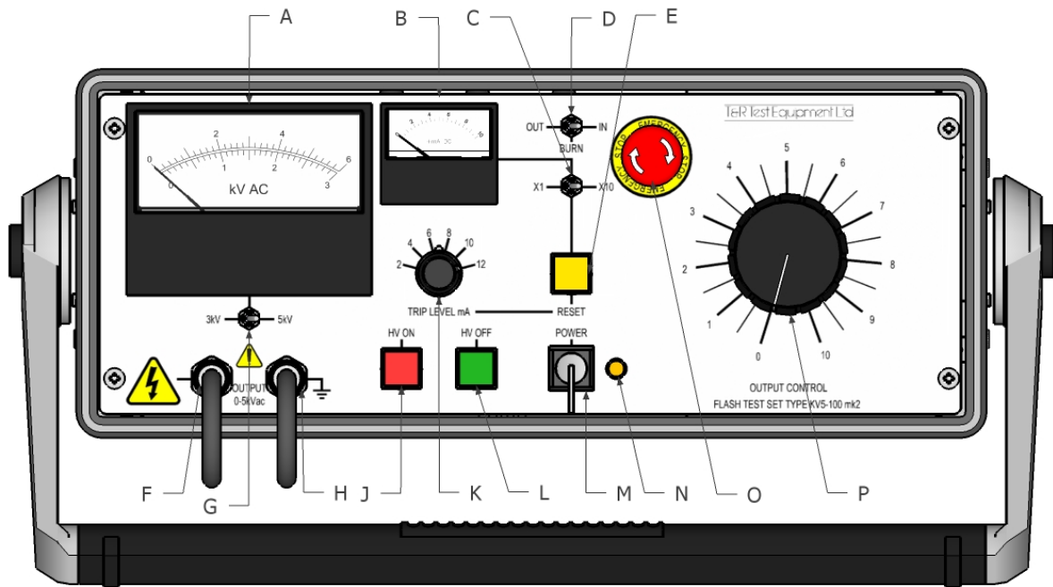
Figure 2.1 KV5-100 mk2 front panel
