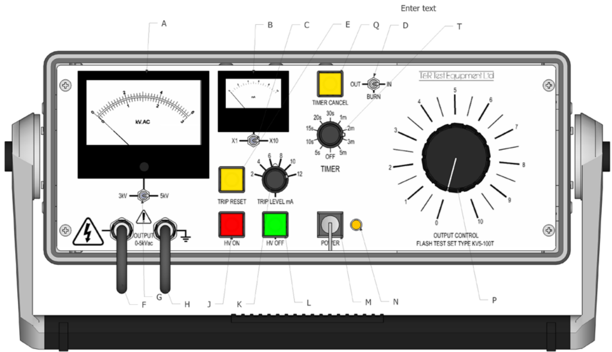
Figure 2.3 KV5-100T front panel
