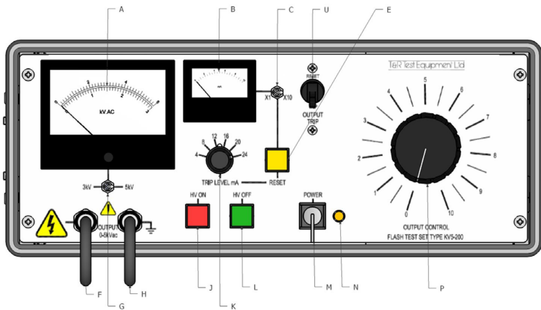
Figure 2.4 KV5-200 front panel
