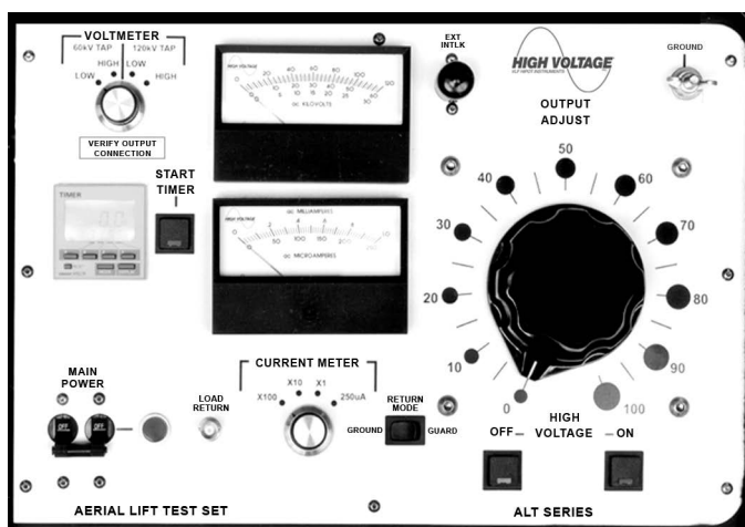
Control Layout
