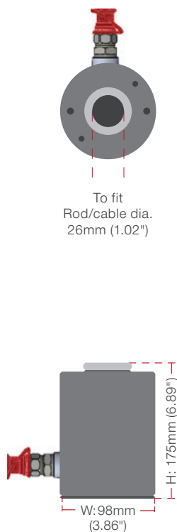
180kN Cylinder
