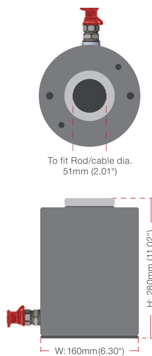
500kN Cylinder
