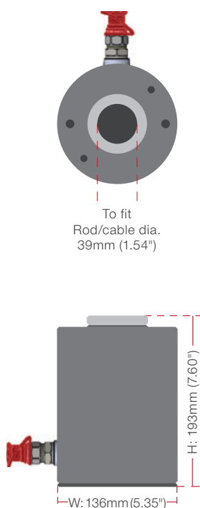
370kN Cylinder
