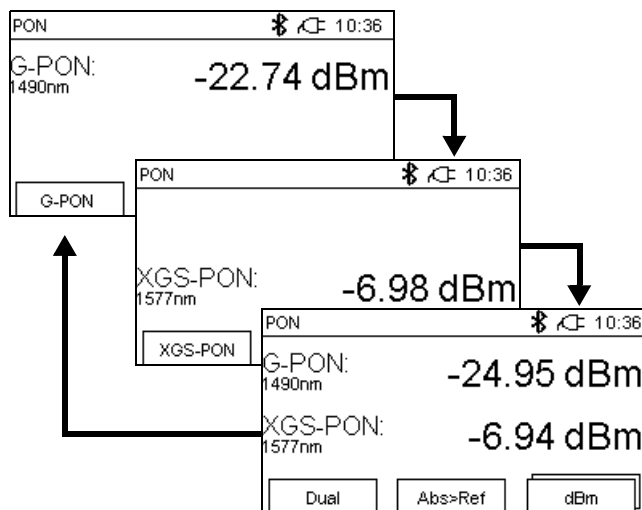
Fig. 4 Operation modes
