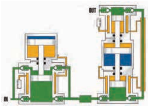
Model AGD-4 feeding into Model AGT-x/x
