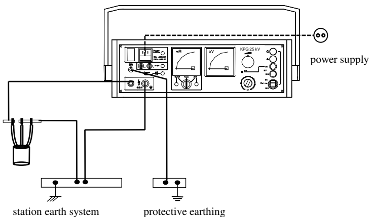
Abb. 3.3 Example for connecting KPG 25 kV
